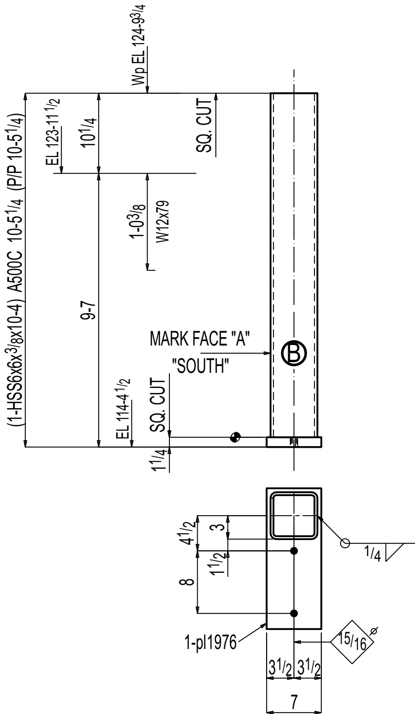
ONE COLUMN F-13.02C1
