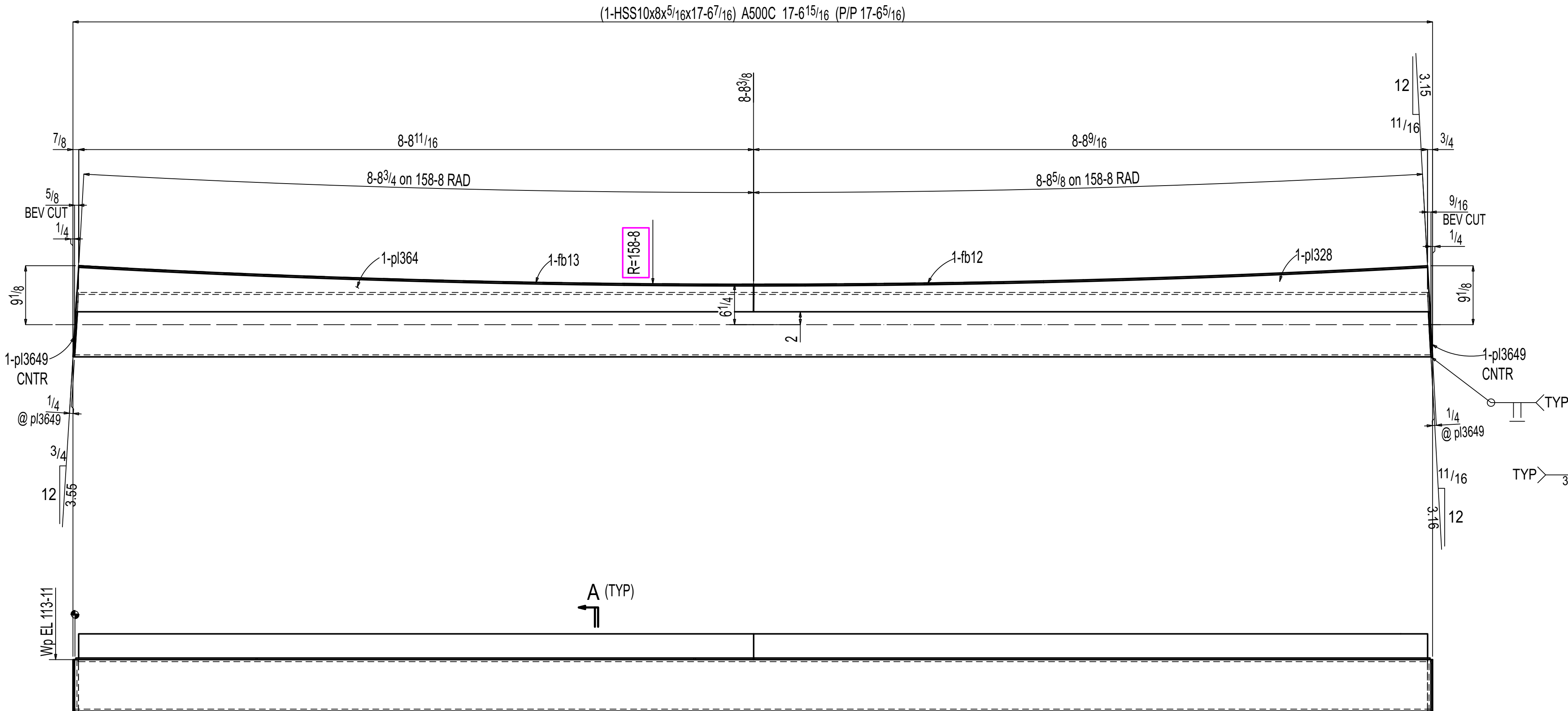
ONE BEAM F-13.02B1
